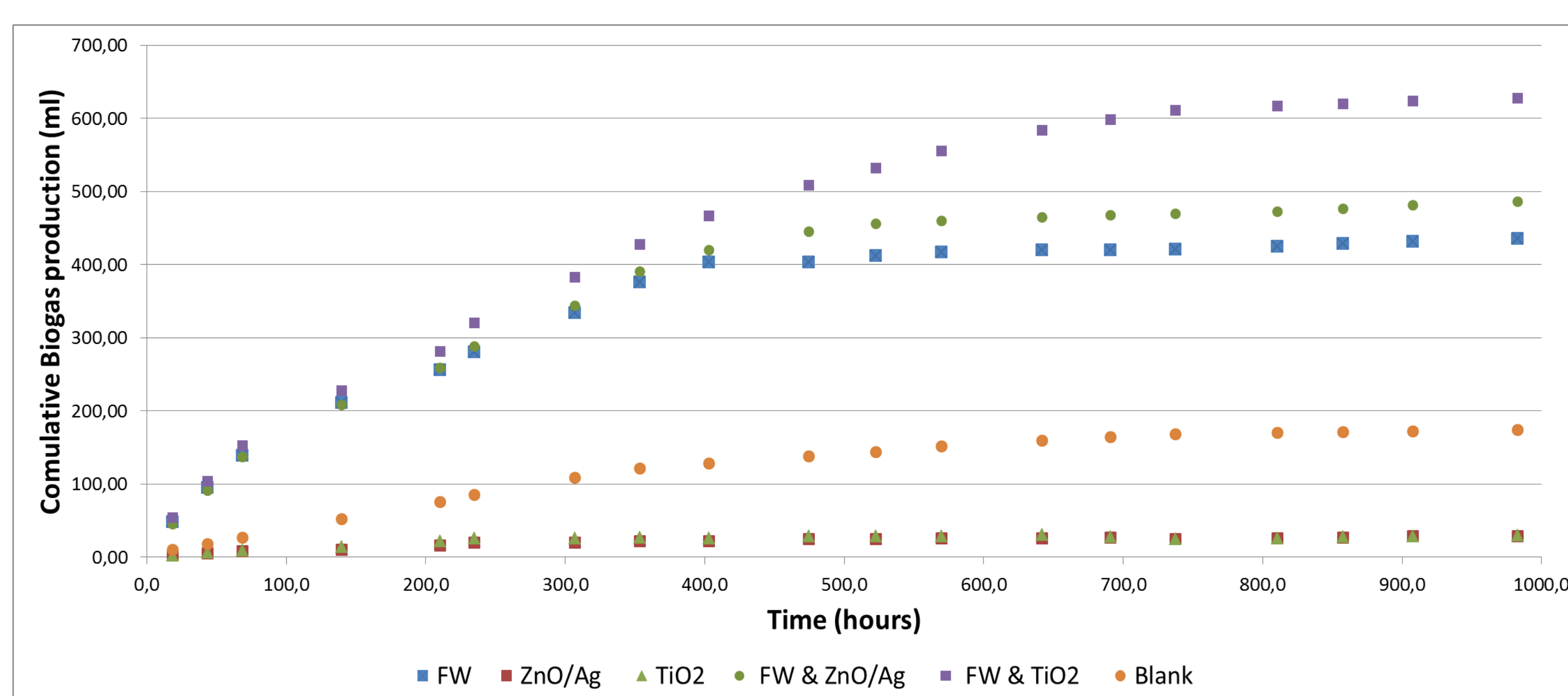
Figure: Cumulative biogas production for different substrate.
