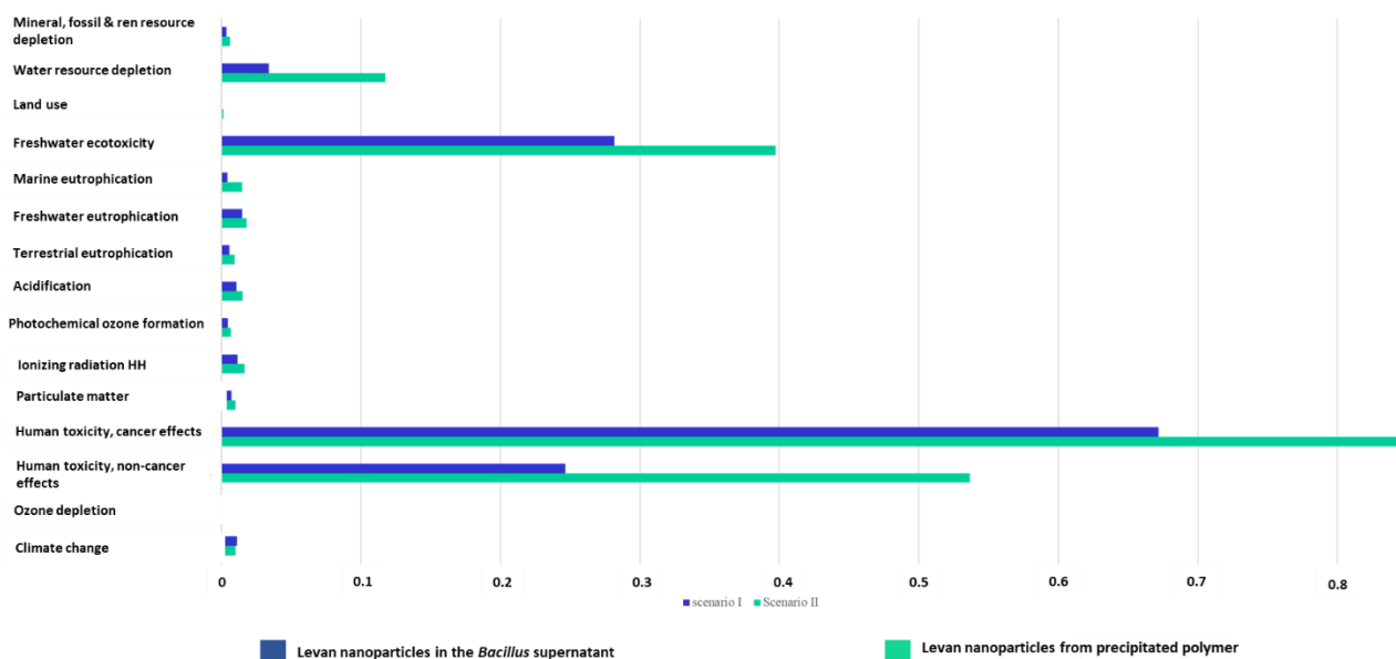
Fig.2 Environmental impact of two different scenarios using ILCD method [Pt] in impact categories
