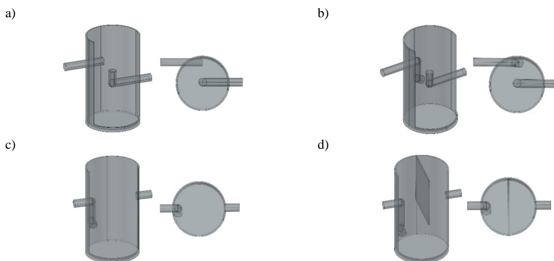
Figure 1. Swirl sedimentation tank:
