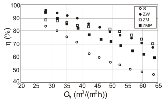
Figure 3. Efficiency of separating solid particles with a diameter of 125 \mu\text{m} from liquid (water) with regards to the hydraulic load for a standard sedimentation tank (S) and its direct modifications (ZW, ZM and ZMP).
