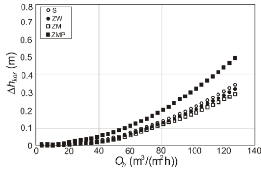
Figure 2. Correlatively determined values of liquid (water) level for the tested structures of the swirl sedimentation tanks.
