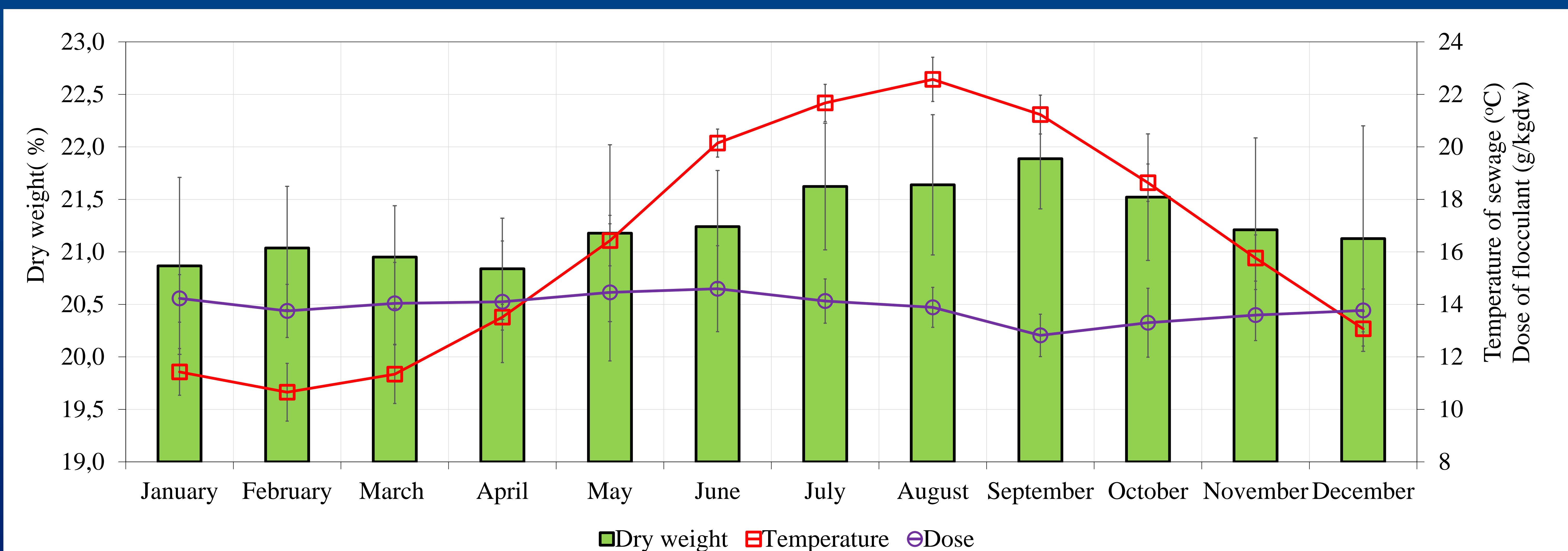
Figure 1. Average values of the dry weight of the cake, waste water temperature and flocculant dose
